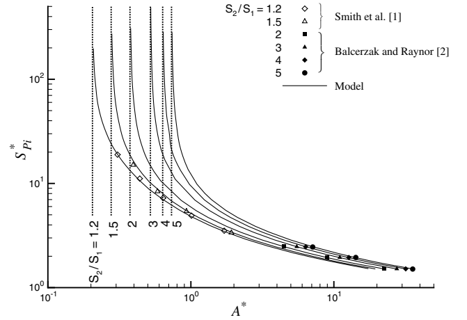
Fig. 7 Model validation for a rectangular cylinder with a concentric circular hole.
